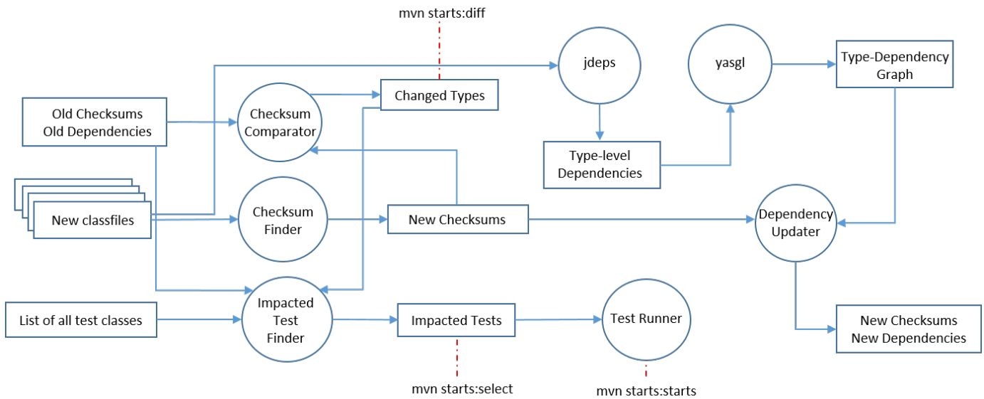
Fig. 1. STARTS Architecture
